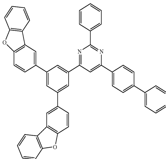
Compound 50
