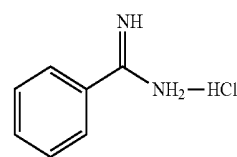
Compound 4
