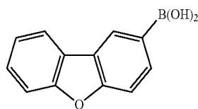
Compound 6
