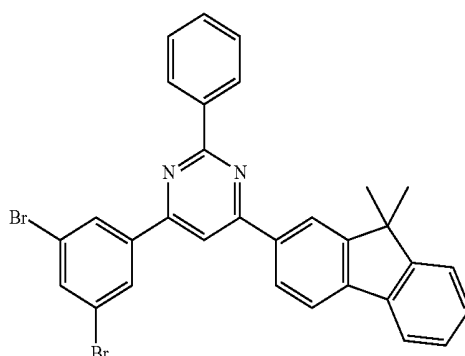
Compound 81
