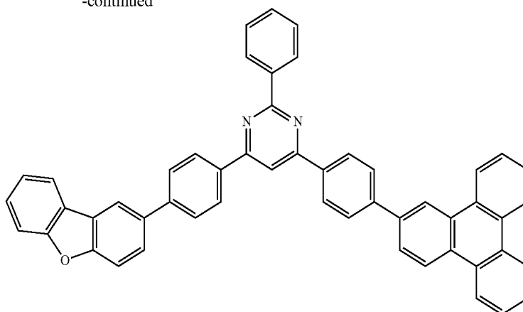
Compound 59
