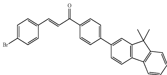
Compound 62
