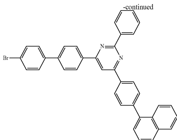
Compound 87
