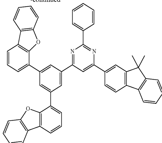
Compound 83
