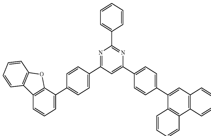
Compound 51
