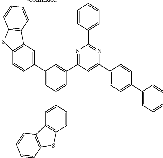
Compound 72
