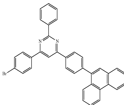
Compound 21
