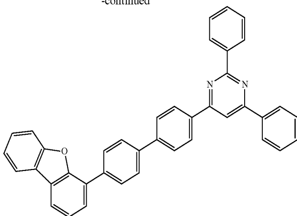
Compound 14
