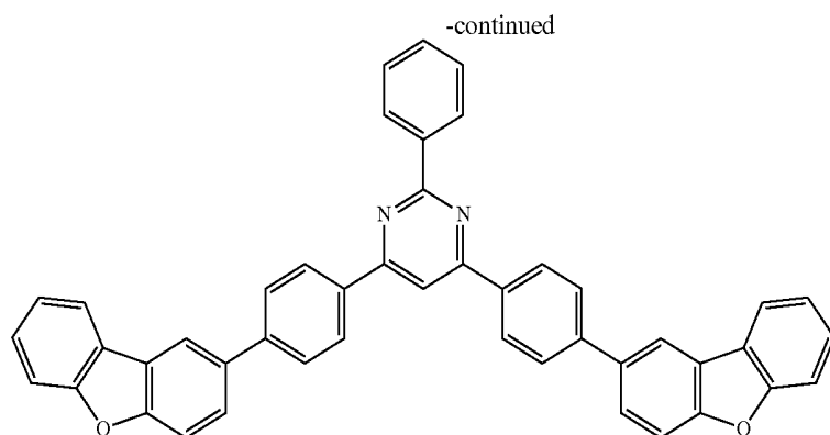
Compound 31
