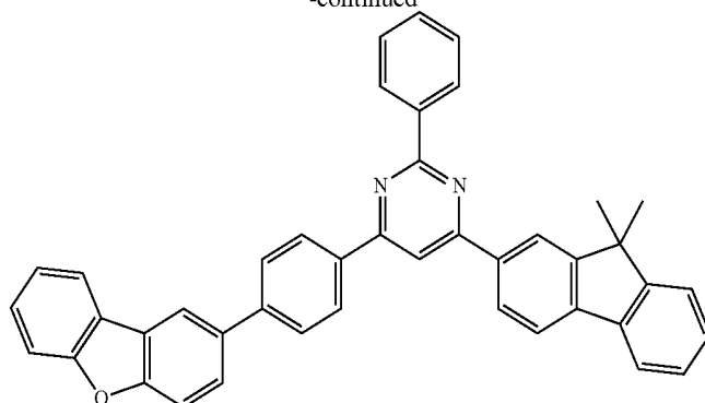
Compound 28
