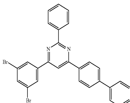
Compound 49
