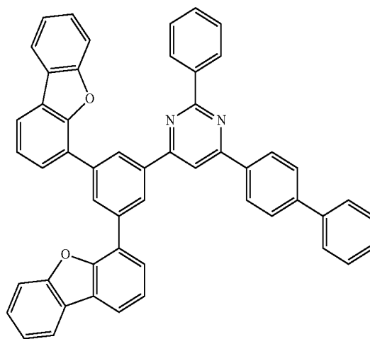
Compound 53
