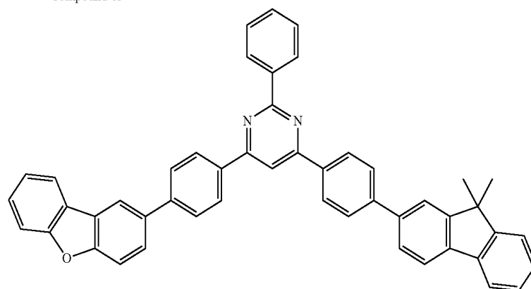
Compound 63
