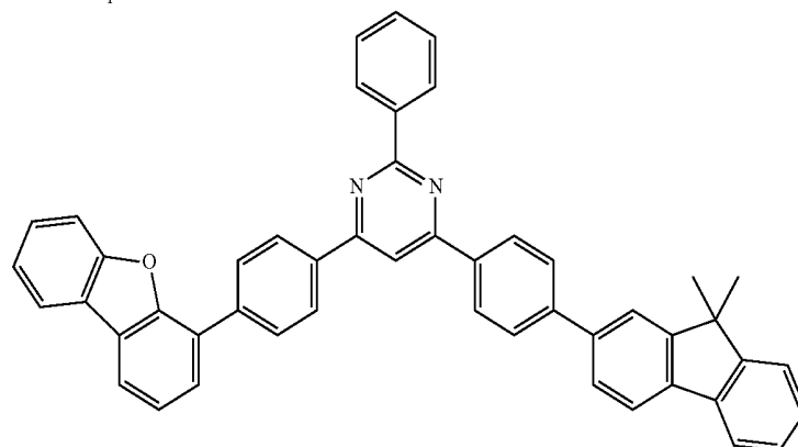
Compound 65
