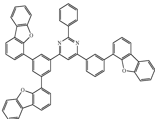
Compound 79
