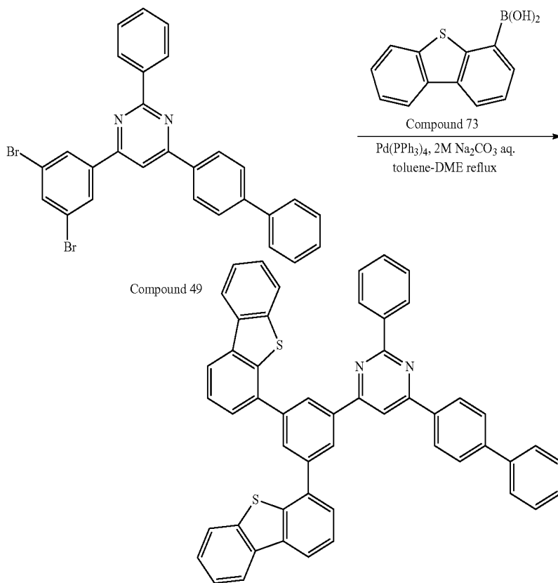
Compound 74
