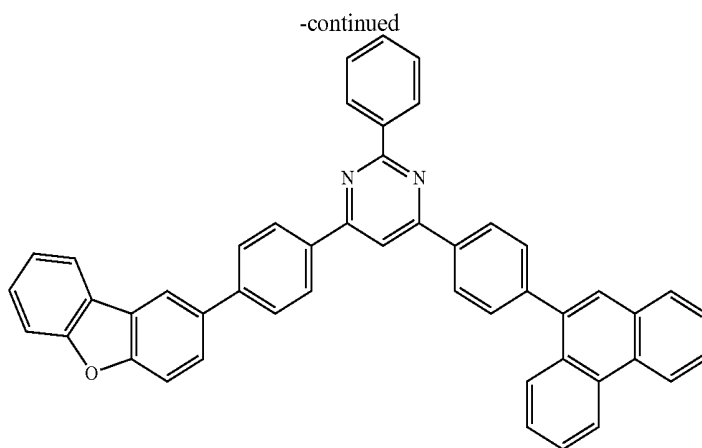
Compound 22
