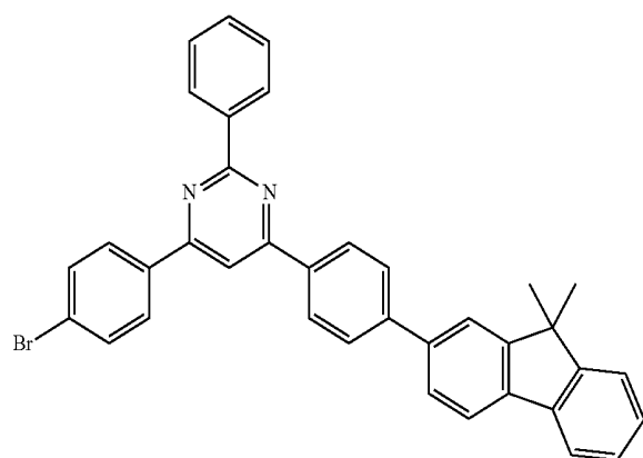
Compound 63
