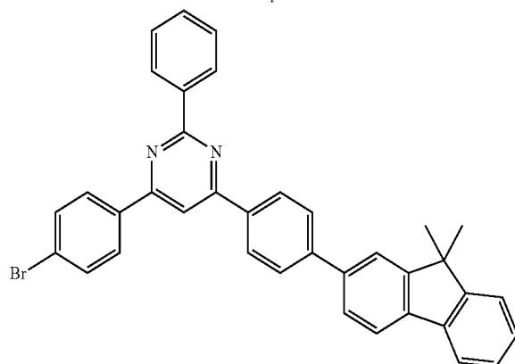
Compound 62
