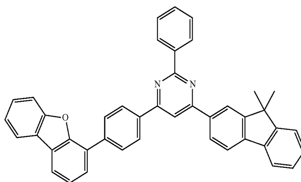
Compound 52
