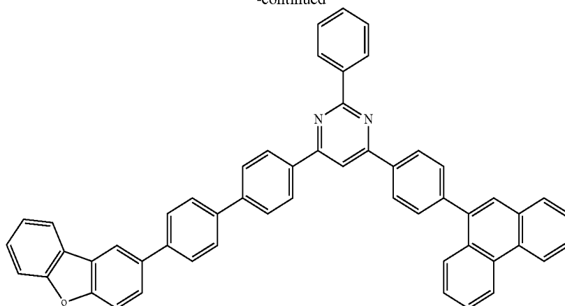
Compound 24
