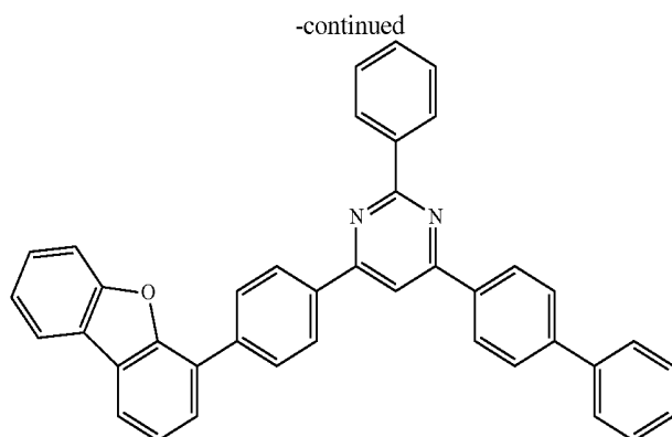
Compound 9
